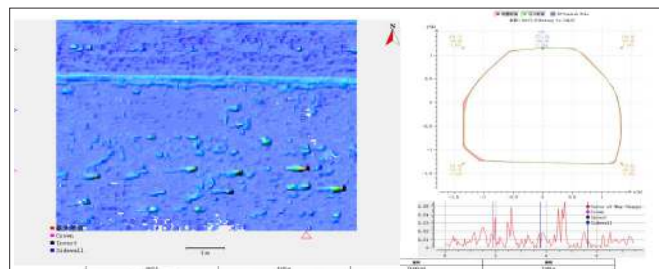
Tunnel Deformation Monitoring
